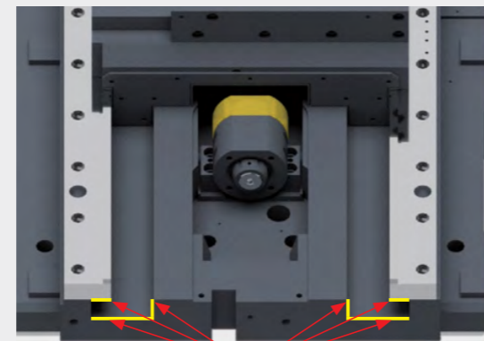
Hexahedral Slide Way Frame
